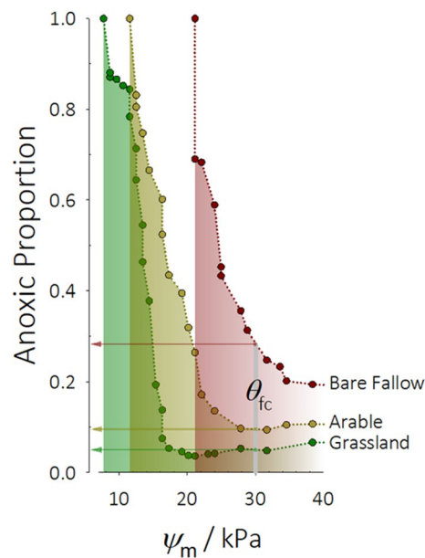
Figure 4. Process-form states control anoxia within soil. Low- C_{org} , low-connected porosity soil contains much larger volumes of anoxic microsities than high- C_{org} , high-connected porosity soil. Across a range of matric potential ( \psi_m ), the predicted volume of anoxic sites is consistently larger in degraded bare fallowed soil than arable or grassland. At field capacity ( \theta_{fc} ), approximately 30% of degraded soil is anoxic, falling to 5% in grassland soil. At 21 kPa degraded soil is completely anoxic while the volume remains between 4–5% in grassland soil. In arable soil 10% of the soil volume is predicted to be anoxic at \theta_{fc} —double that in grassland.
