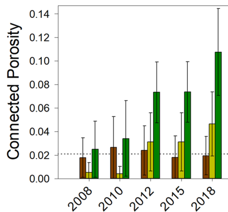
Figure 1. Grassland soils generate connected pore space more rapidly than arable soils. Degraded soil (managed as bare fallow since 1959) developed greater connected micro-porosity following conversion in 2008 to grassland than bare fallow soil converted to arable. The mean and standard error of the mean of connected porosity measured in soil aggregates collected from soil managed continuously as bare fallow (brown), soil converted to arable management (dark yellow) and soil converted to grassland (green) over the ten years following conversion are shown. The dotted line marks the mean connected porosity of continuously managed bare fallow soil over the entire ten-year period.
